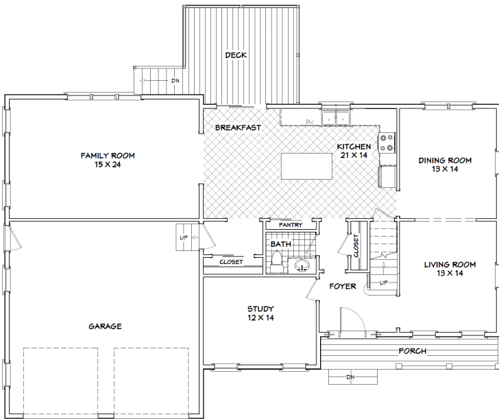
1st Floor
